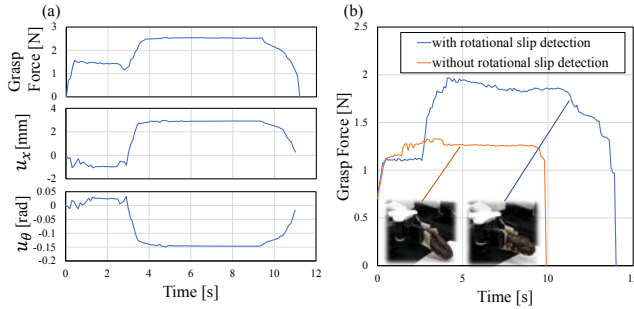
Figure 10. (a) Grasp force \tau , shear displacement u_x and u_\theta when grasping the rectangular plastic bottle, (b) Grasp force with and without rotational slip detection when grasping an éclair.
