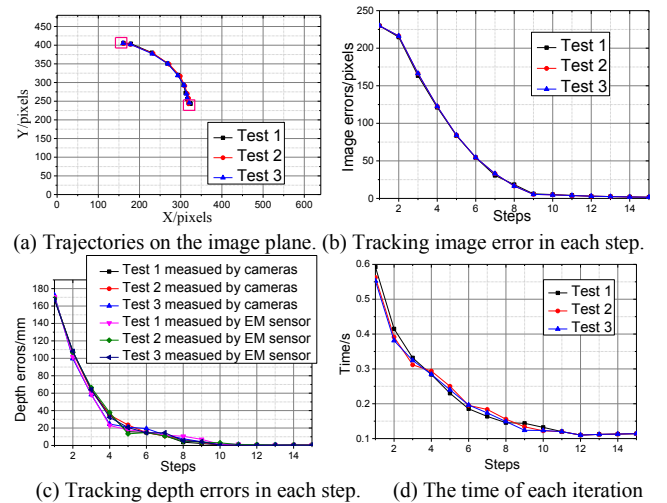
Figure 5. Stationary target tracking results. (a) The pink points are the initial and the desired image positions, respectively. The blue, red and black lines are the trajectories of the three tests. (b) The blue, red and black lines are the image errors of each step in the three tests, respectively. (c) The blue, red and black lines are the target’s depth information of each step in the three tests measured by two cameras, respectively. The blue, red and black dotted lines
