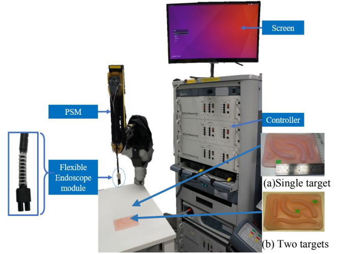
Figure 4. Experimental platform.
