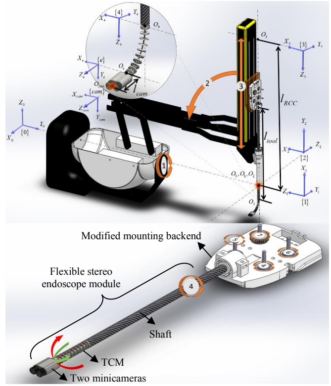
Figure 1. The structure of the proposed RSFE and the coordinate frames for kinematics modelling.
